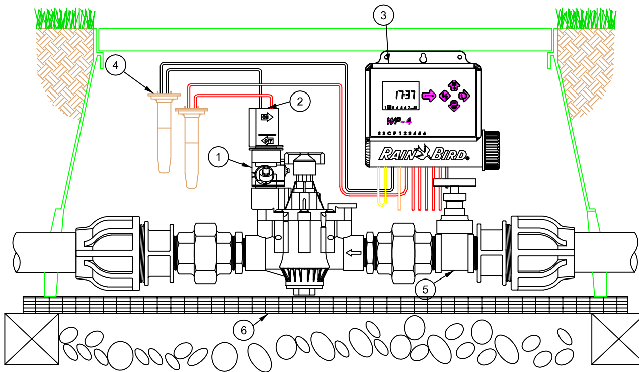
Electroválvula PGA + PRS-Dial / WP-2/4/6/8
