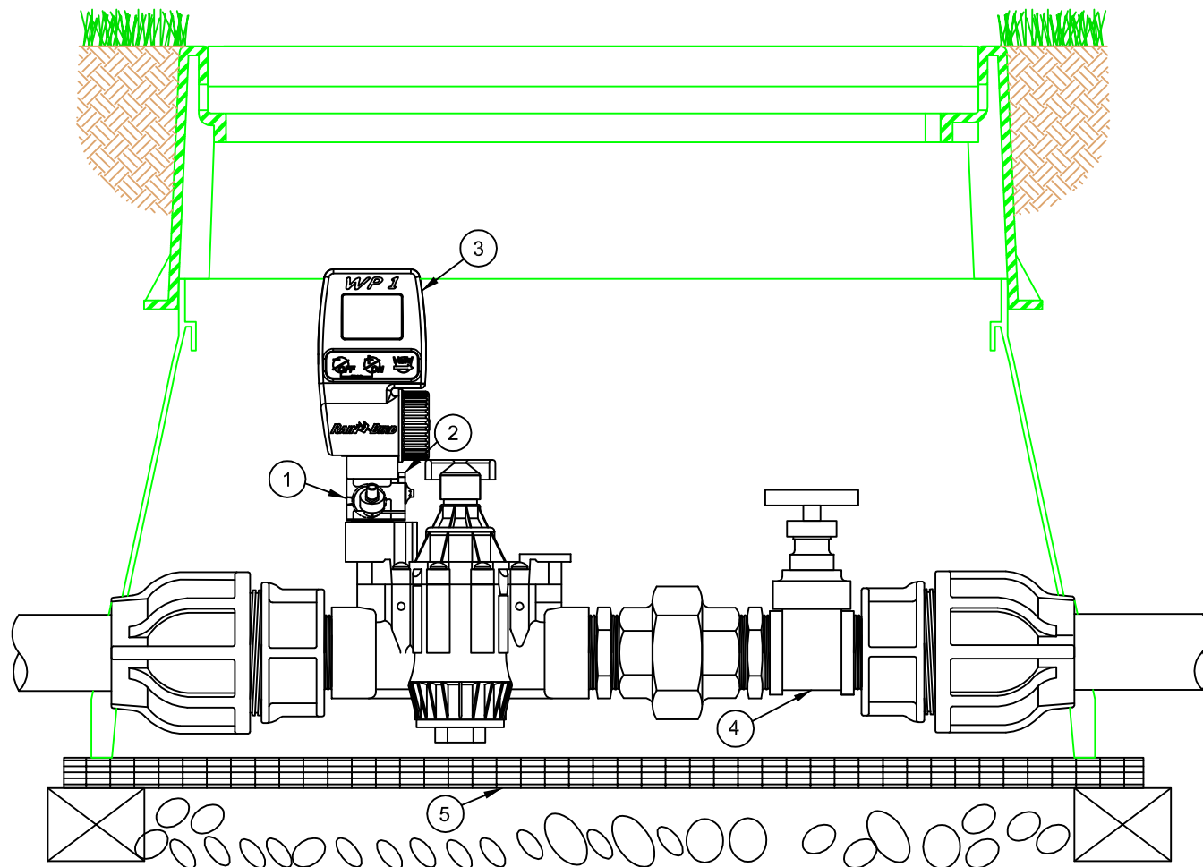
Electroválvula PGA + PRS-Dial / WP-1
